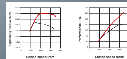
BASIS: Audi TT Coupé 3.2 V6; 250 hp, 320 Nm
