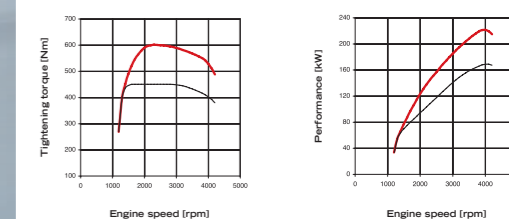
BASIS: AUDI A6 3.0 I TDI; 133 hp, 450 Nm
